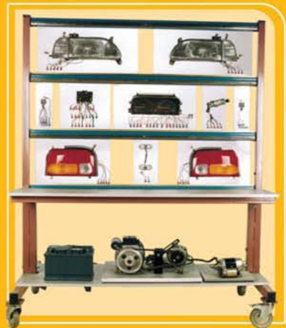
Automobile electrical training set
